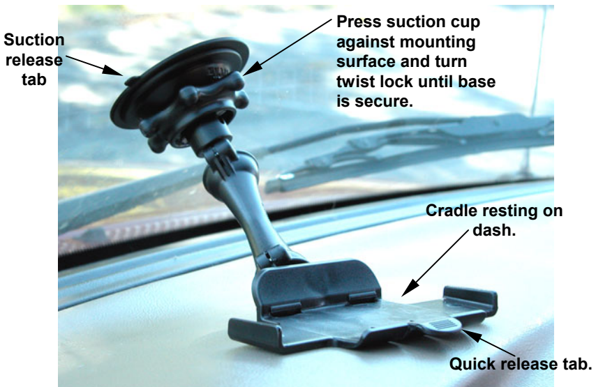
RAM suction cup base secured to windshield ready to accept GPS unit.
